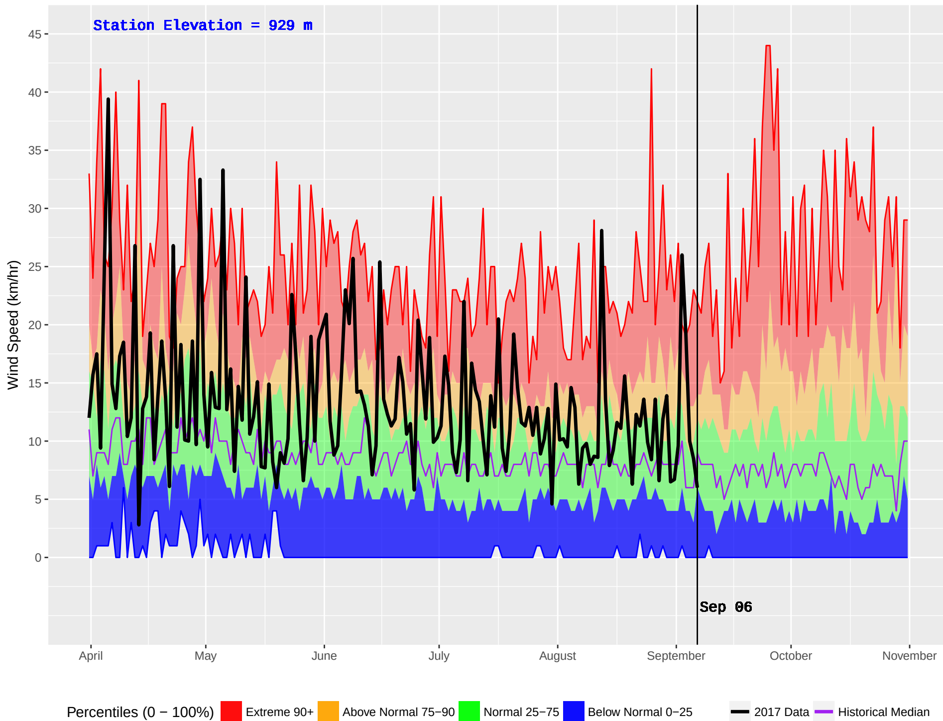
RISKE CREEK (210) : Historical (1980–2016) and Current (2017) Noon Wind Speed
