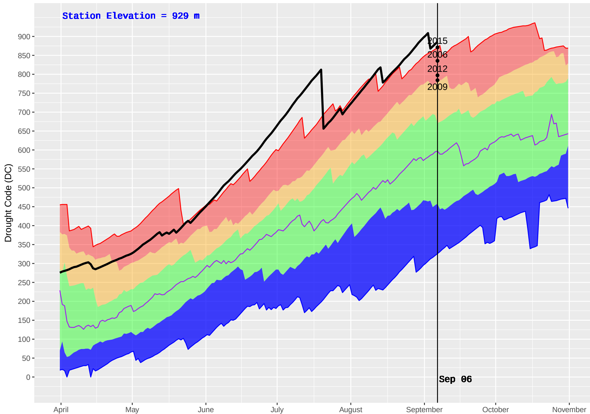
RISKE CREEK (210) : Historical (1980–2016) and Current (2017) Noon Drought Code (DC)
