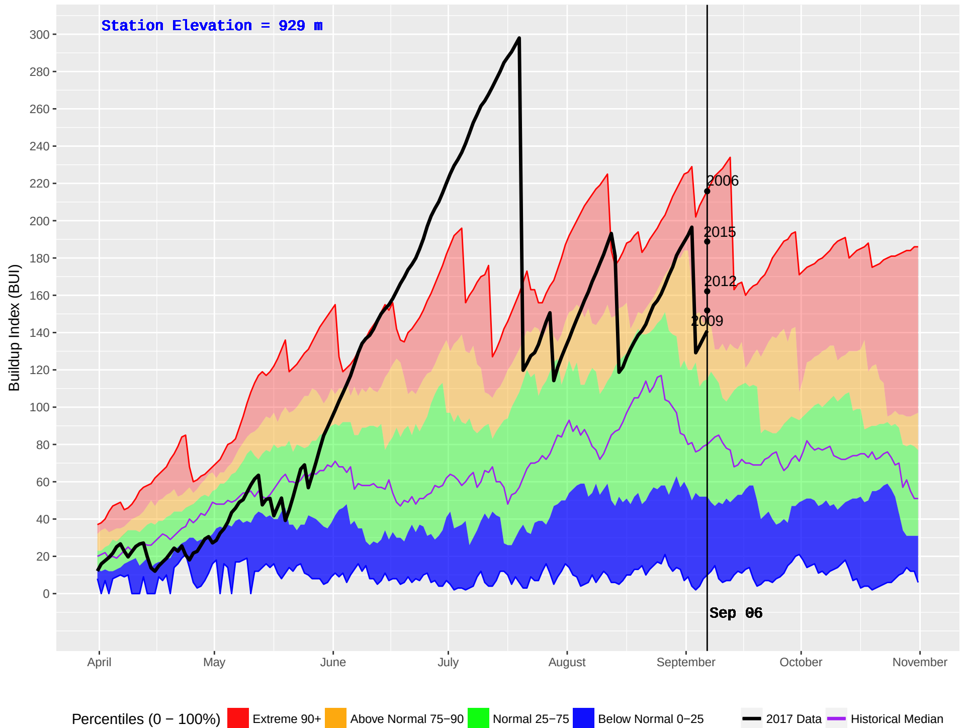
RISKE CREEK (210) : Historical (1980–2016) and Current (2017) Noon Buildup Index (BUI)
